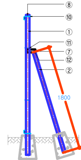
SIDE ELEVATION SCALE : NONE
