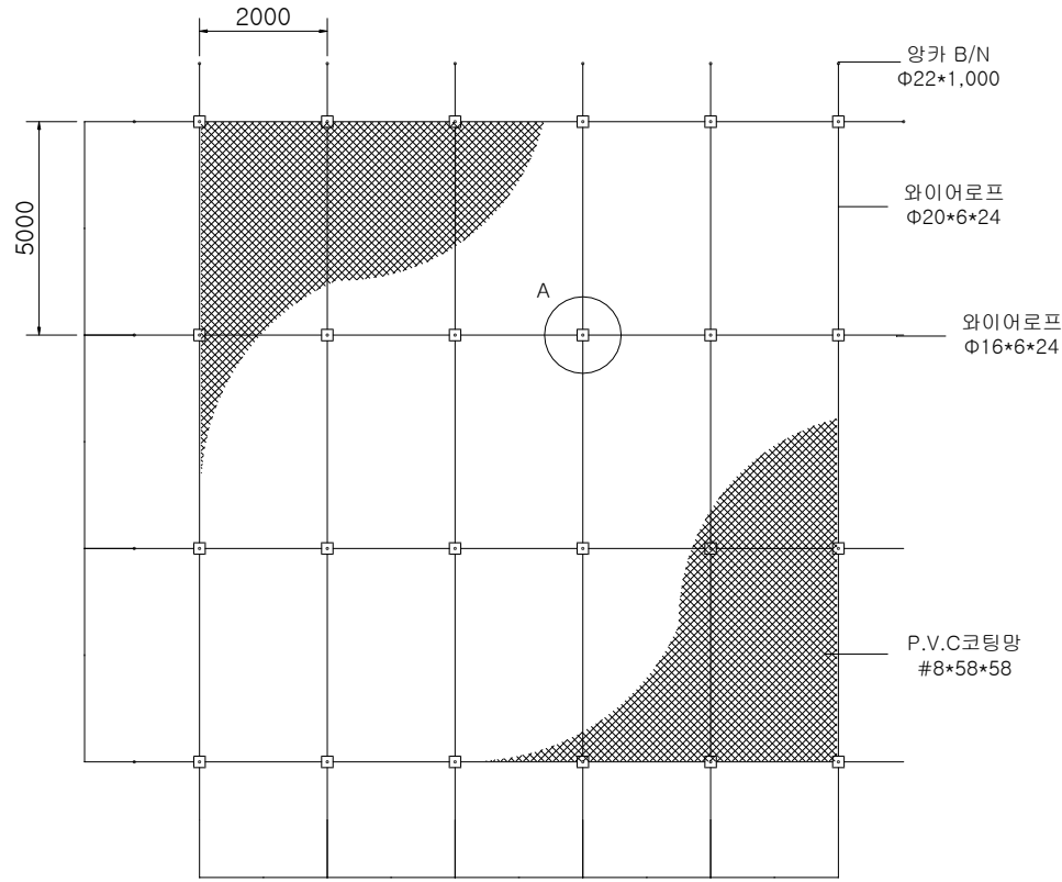
ELEVATION SCALE : NONE
